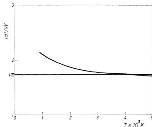
Fig. 3. Shift-to-half-halfwidth ratio for HeI( 3^1P^0-2^1S ).
